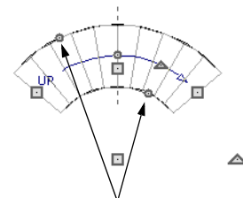
Adjust Width
